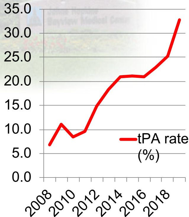
tPA rate (%)
